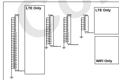
SMD Shieldcan
