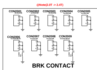
BRK CONTACT
